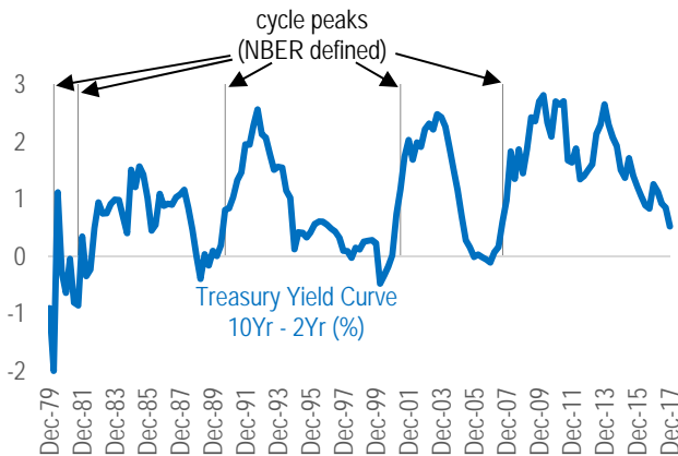
Chart 7: Yield Curve
